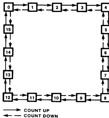
STATE DIAGRAM
