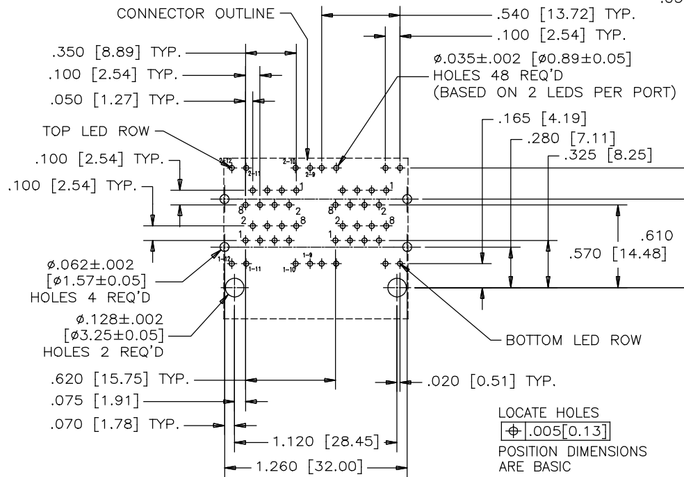
RECOMMENDED P.C.B. LAYOUT (COMPONENT SIDE OF BOARD) TOLERANCE: ±0.05 [0.02]
