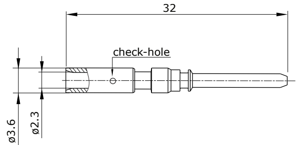
Main Dimensions contact pin
