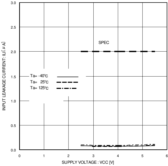
Figure 11. Input Leakage Current ILI (GSB,SCK,SI,HOLDB,WPB)
