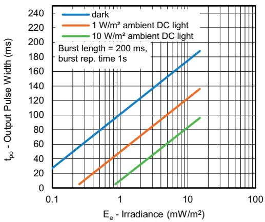
Fig. 6 - Max. Output Pulse Width vs. Irradiance
