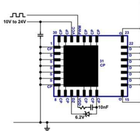
Fig. 18. Start-up circuit
