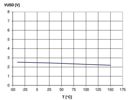
Figure 19: Undervoltage shutdown
