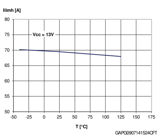
Figure 26: Ilimh vs. Tcase
