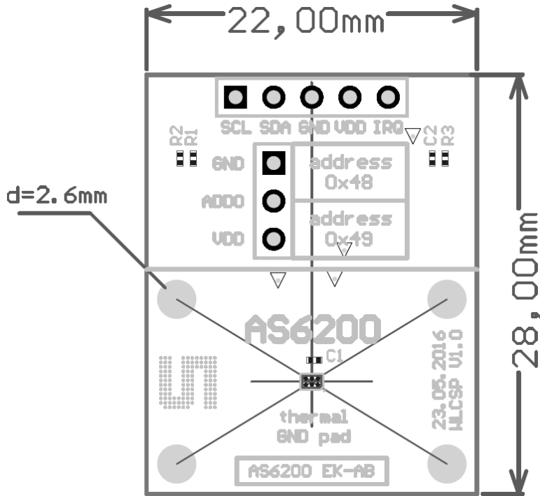
Figure 7: Dimensions
