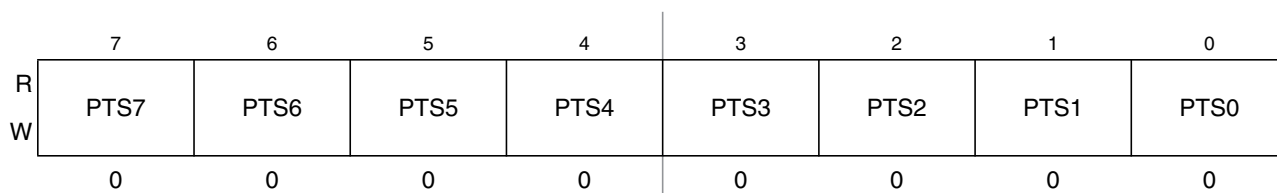
Figure 2-21. Port S Data Register (PTS)
