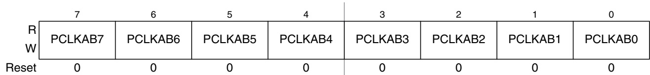
Figure 19-9. PWM Clock Select Register (PWMCLKAB)
