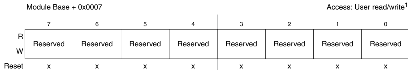
Figure 17-5. Reserved Registerfv_dac_8b5v_RESERVED
