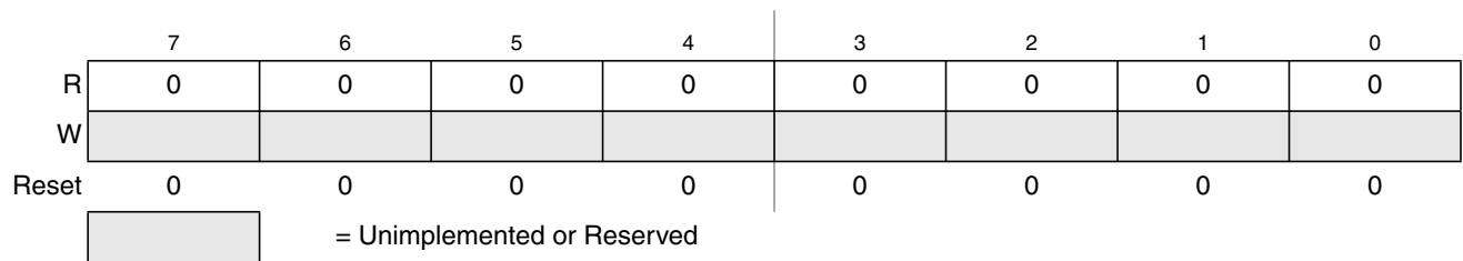
Figure 25-21. Flash Reserved4 Register (FRSV4)
