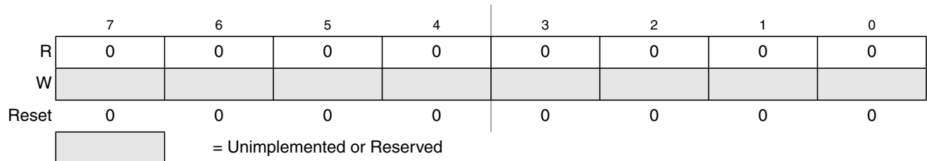
Figure 24-17. Flash Reserved1 Register (FRSV1)
