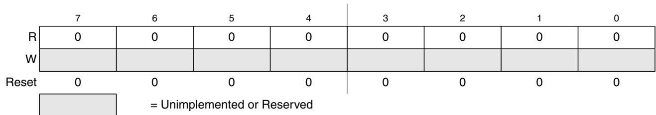
Figure 30-8. Flash Reserved0 Register (FRSV0)
