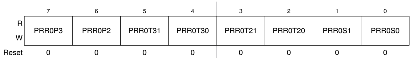
Figure 2-27. Pin Routing Register (PRR0)
