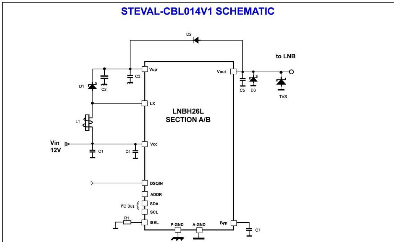
Figure 1: STEVAL-CBL014V1 schematic
