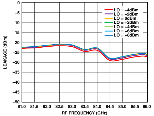
Figure 56. 6x LO Leakage at RFOUT vs. RF Frequency at Various LO Powers, IFIN = 5 dBm, IF = 500 MHz, LSB
