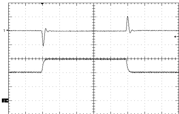
Figure 11. Load Transient Response (100mV/div), di/dt=0.1A/uS, 50% - 75% - 50% of full load, time scale: 200uS/div. Ch2=2A/div
