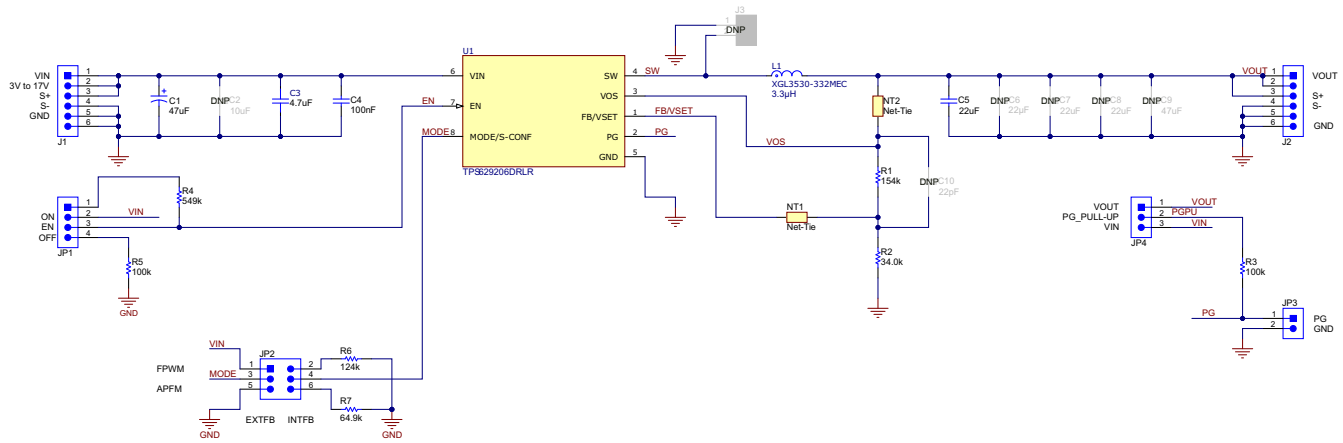
Figure 7-1. TPS629206EVM Schematic
