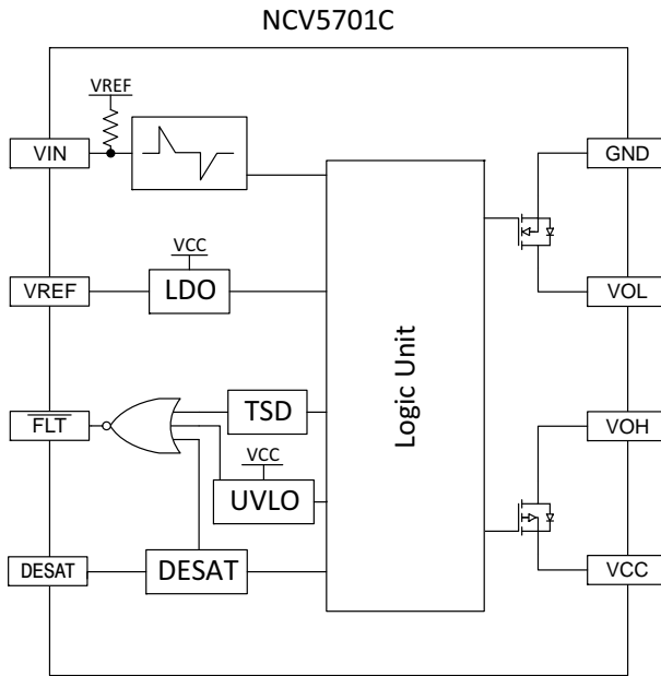
Figure 4(b). Simplified Block Diagram NCV5701C
