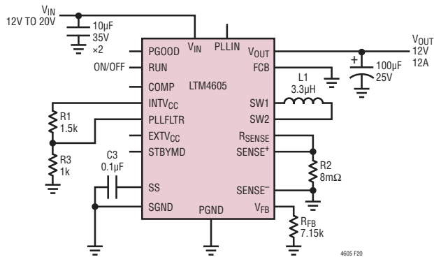
Figure 20. Buck Mode Operation with 12V to 20V Input
