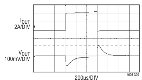
Transient Response from 18V IN to 12V OUT
