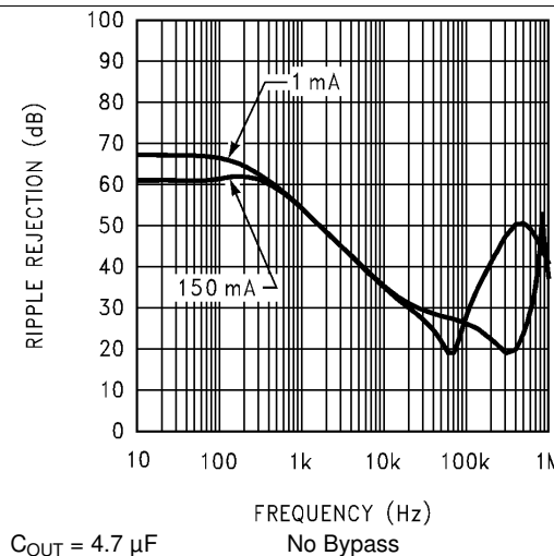
Figure 6. Ripple Rejection
