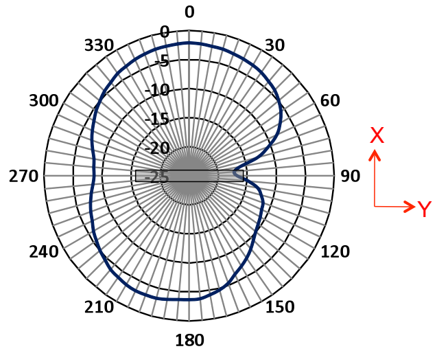
Figure 6b: Radiation diagram of X-Y plane shows combined polarizations at 635 MHz
