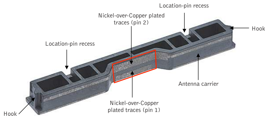
Figure 1. Design features of a Mobile TV Standard Antenna
