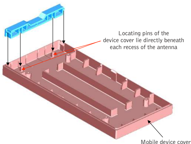
Figure 2. Alignment and interlocking features of the antenna and mobile device cover
