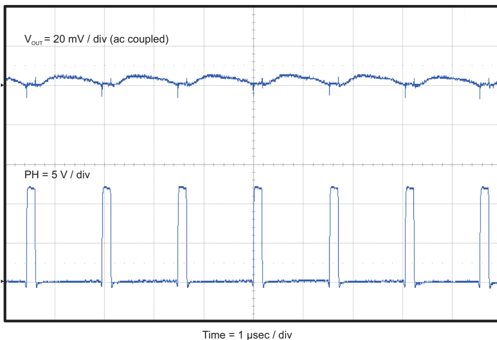
Figure 4-6. TPS54229EVM-056 Output Voltage Ripple
