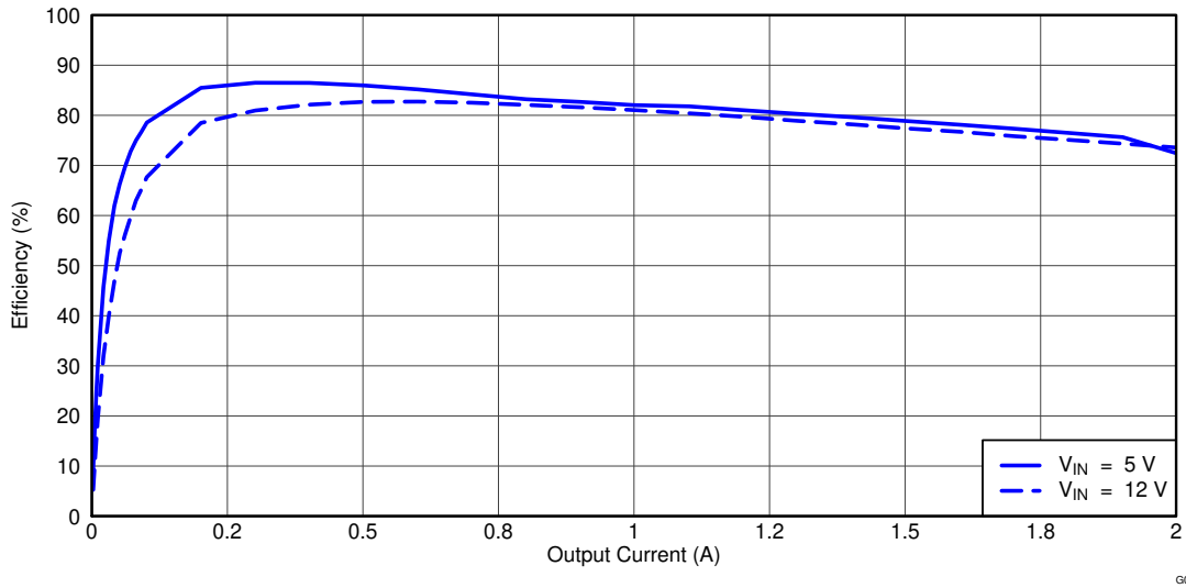
Figure 4-1. TPS54229EVM-056 Efficiency
