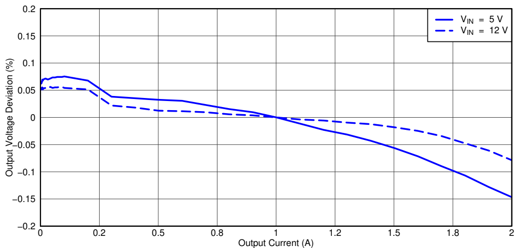
Figure 4-3. TPS54229EVM-056 Load Regulation, V_{IN} = 5V and V_{IN} = 12V .
