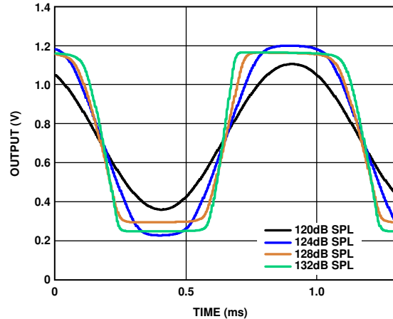
Figure 8. Clipping Characteristics
