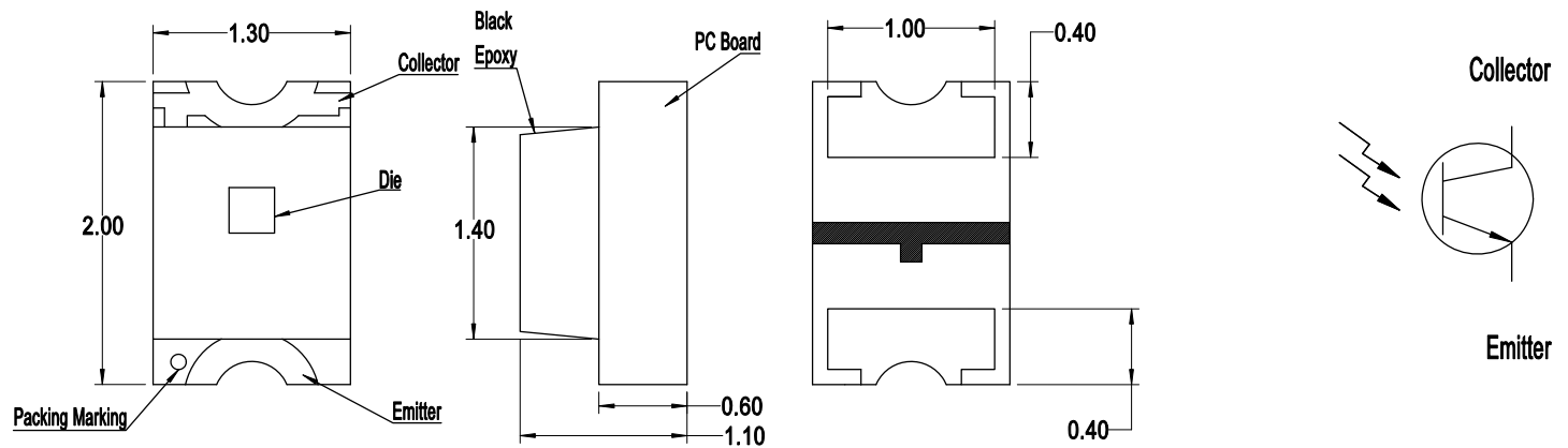
Figure 1: Package Drawing
