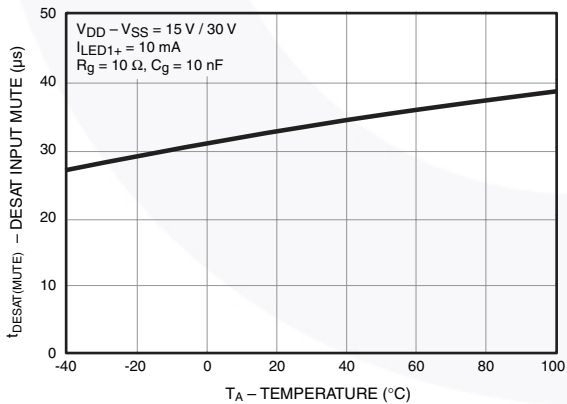
Figure 27. DESAT Input Mute ( t_{DESAT(MUTE)} ) vs. Temperature
