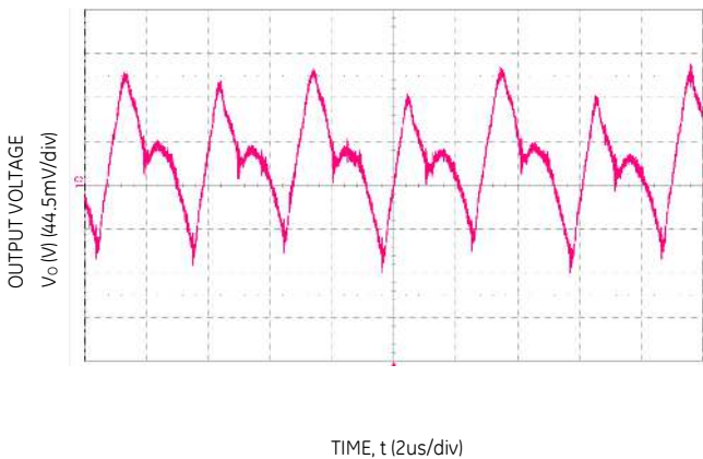
Figure 9. Typical output ripple and noise ( C_o=3 \times 10\mu F+470\mu F , V_{IN} = 12V , I_o = I_{o,max} ).
