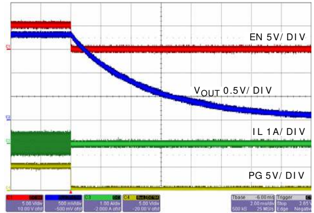
FIGURE 28. SOFT-DI CHARGE SHUTDOWN
