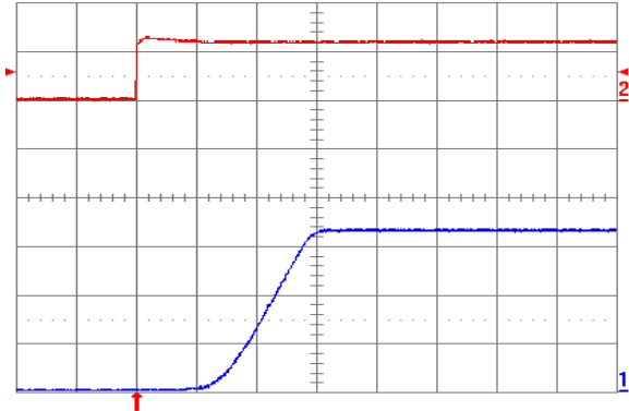
Fig. 3.3V.5: Turn-on transient for V_{out} = 3.3V with application of V_{in} = 12V at full rated load current (resistive) and 47\mu F external capacitance. Top trace: V_{in} (10V/div); Bottom trace: V_{out} (1V/div); Time scale: 2 ms/div.
