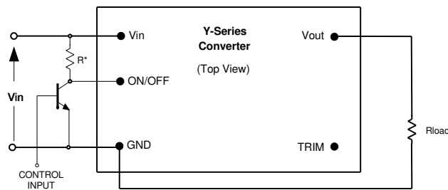
Fig. A: Circuit configuration for ON/OFF function.
