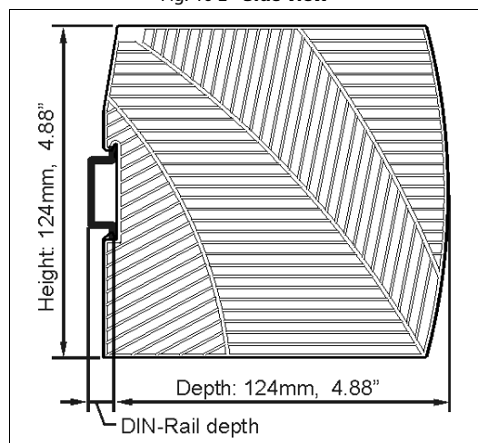
Fig. 16-2 Side view
