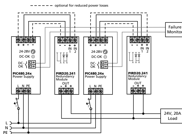
Fig. 17-4 Wiring diagram, 1+1 Redundancy, 20A output current
