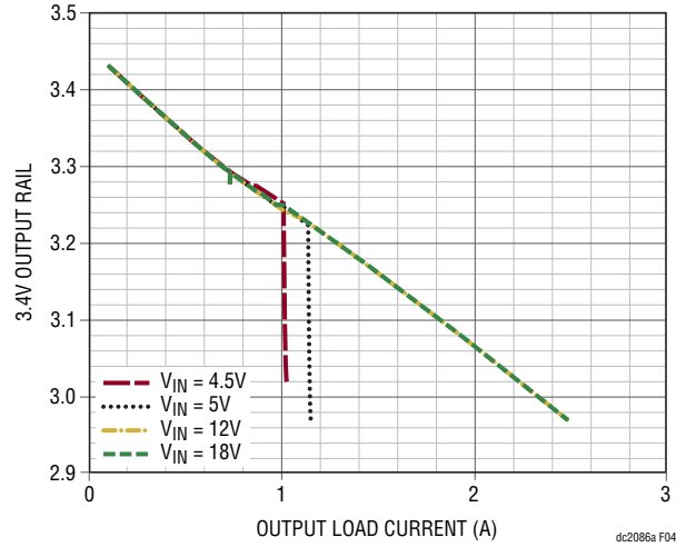
Figure 4. 3.4V V OUT vs I OUT
