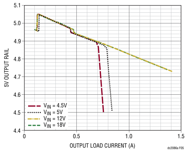
Figure 5. 5V V OUT vs I OUT
