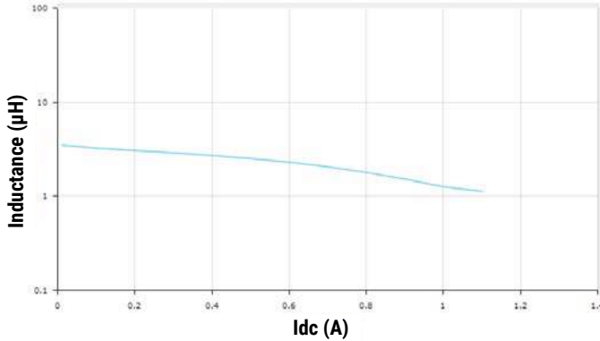
L1008Q3R3MDMIT
