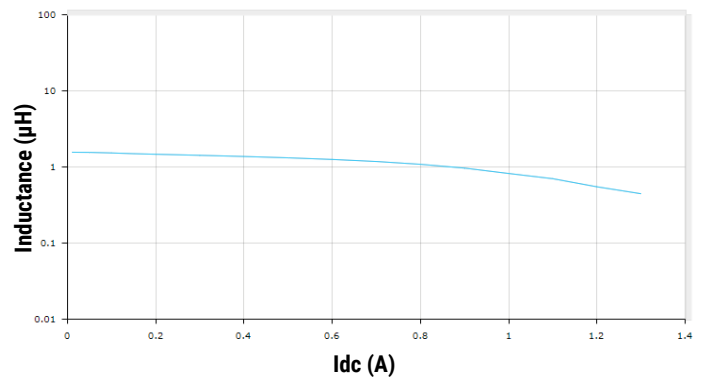
L1008L1R5MDMIT
