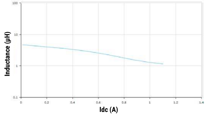
L1008Q4R7MDMIT
