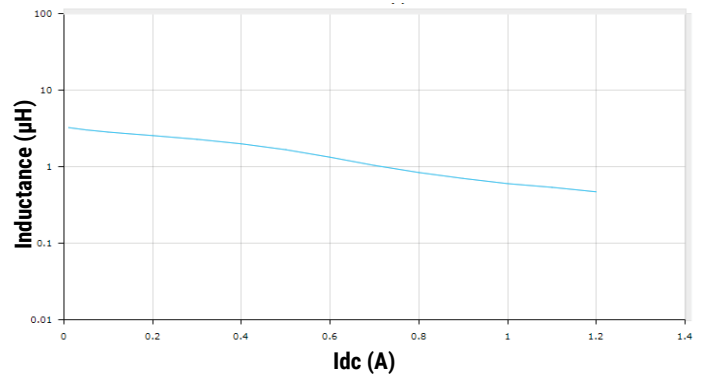
L1008C3R3MDMIT
