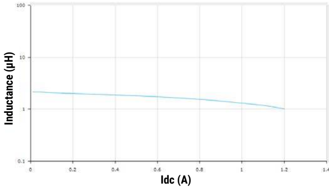
L1008S2R2MDMIT
