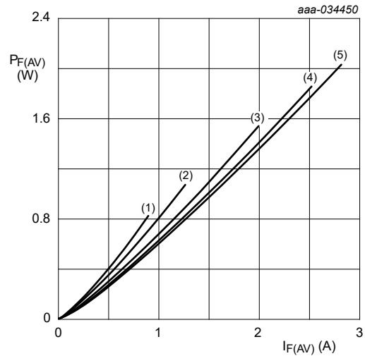
T_j = 100\text{ }^\circ\text{C} (1) \delta = 0.1 (2) \delta = 0.2 (3) \delta = 0.5 (4) \delta = 0.8 (5) \delta = 1; \text{DC}
