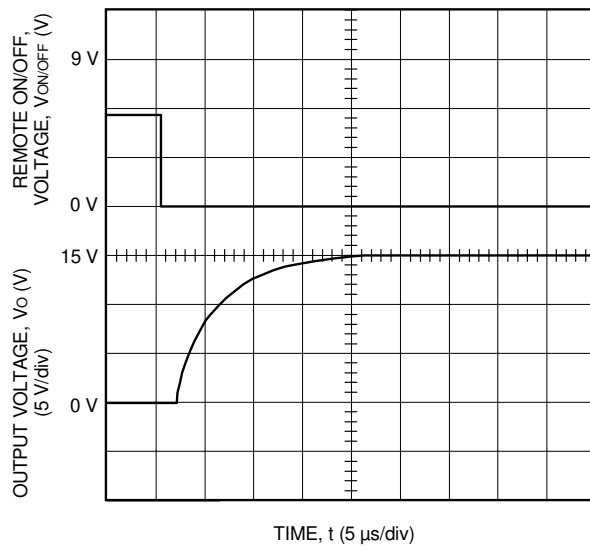
Figure 10. Typical Start-Up from Remote On/Off JC100C1; Io = Full Load
