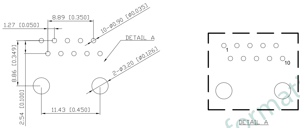
SUGGESTED PCB LAYOUT (TOP VIEW) SCALE:2:1 DIMENSIONAL TOLERANCE: .XX ±0.08[0.003]
