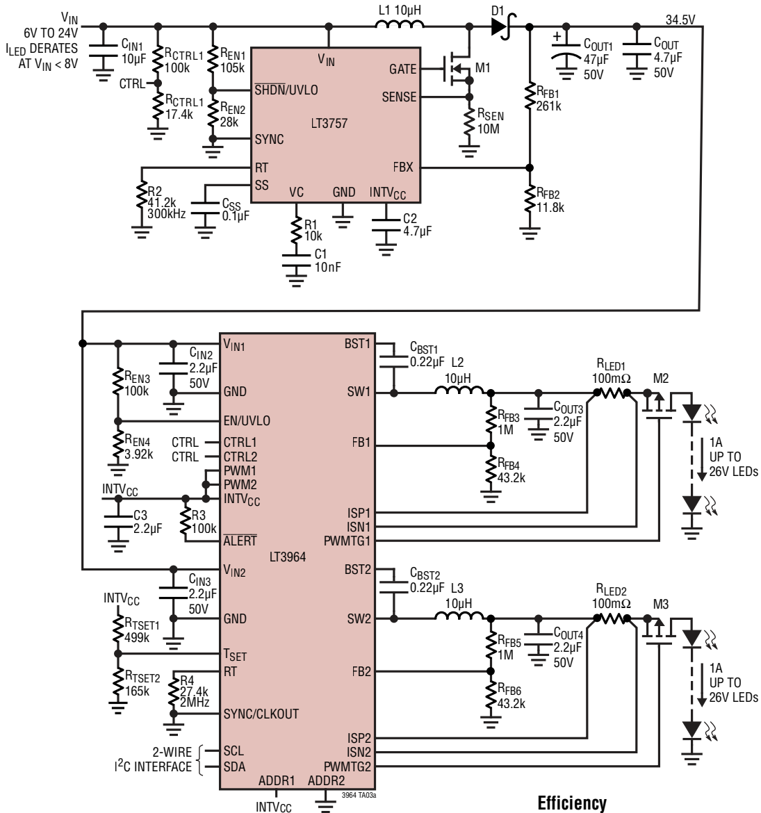
Multi-Channel Boost Buck LED Driver
