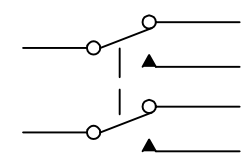
CIRCUIT DIAGRAM (DPDT) ON-MOMENTARY
