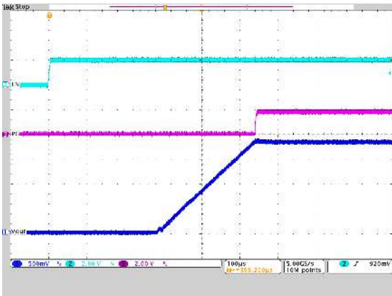
Figure 9-20. Start-Up Timing
