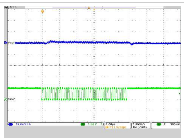
Figure 9-25. Frequency Synchronization
