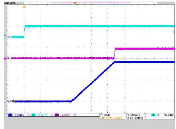
Figure 9-21. Start-Up Timing
