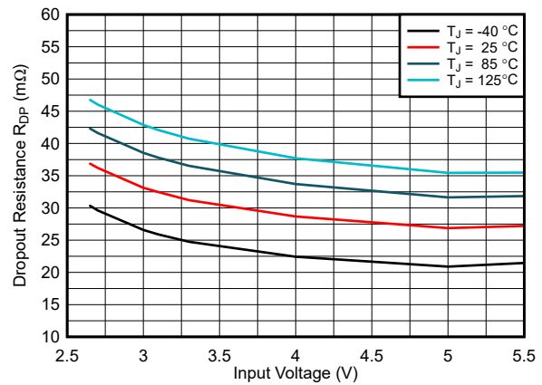
Figure 7-4. Dropout Resistance
