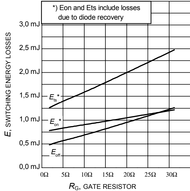
Figure 14. Typical switching energy losses as a function of gate resistor (inductive load, T_J=150^{\circ}\text{C} , V_{CE}=400\text{V} , V_{GE}=0/15\text{V} , I_C=30\text{A} , Dynamic test circuit in Figure E)
