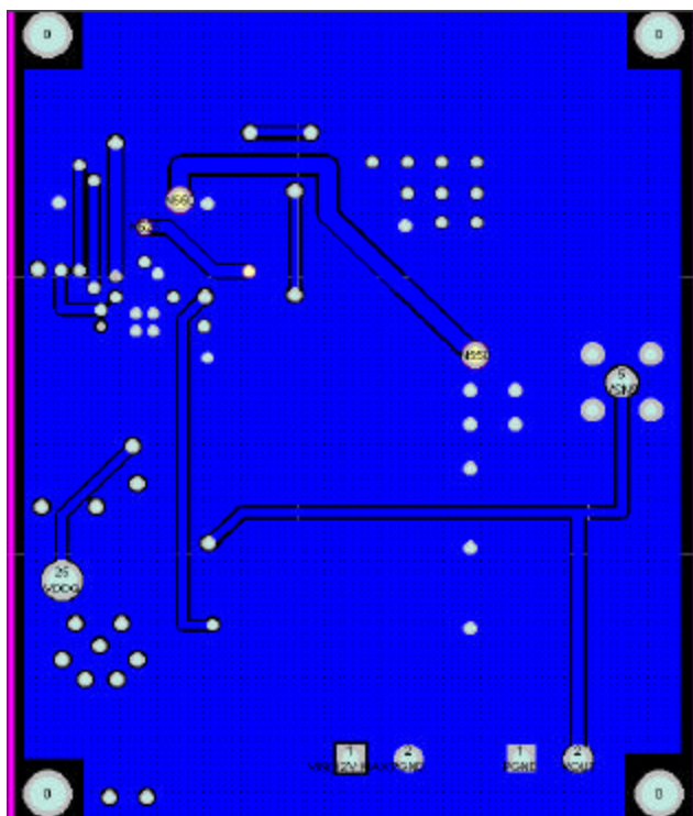
Figure 2.4 - Bottom layer.
