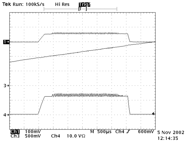
Figure 8 - Output shorted at start up. Ch1: V_{OUT} , Ch3: V_{ss} , Ch4: Inductor Current
