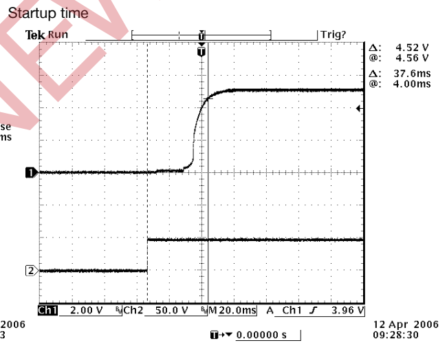
CH1: Vout CH2: Vin Vout=5V 100% Load at Vin=48V
