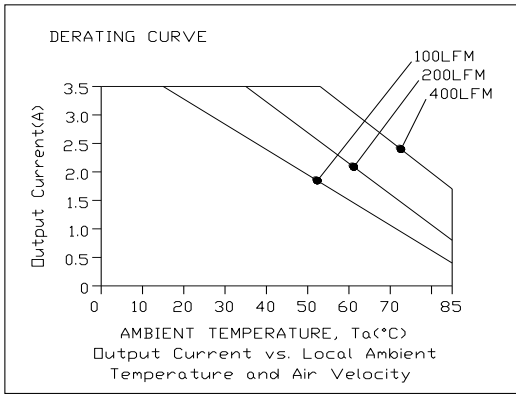
xRSB-40U12x, Vin=18V
