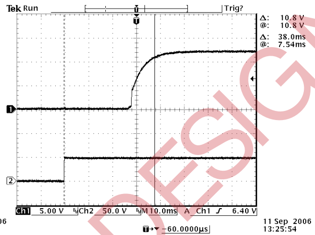
Startup time
