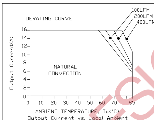
xRSB-40UV5x, Vin=75V
