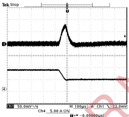
Vout=1.5 V 50% to 25% Load Transients
