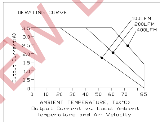
xRSB-40U12x, Vin=24V
