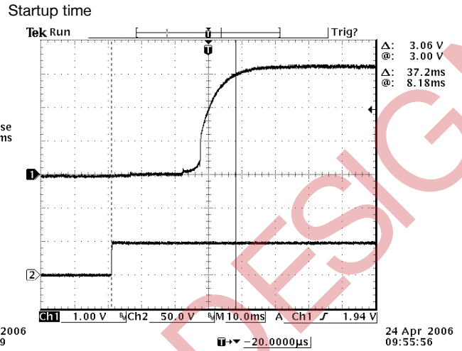
CH1: Vout CH2: Vin Vout=3.3V 100% Load at Vin=48V
