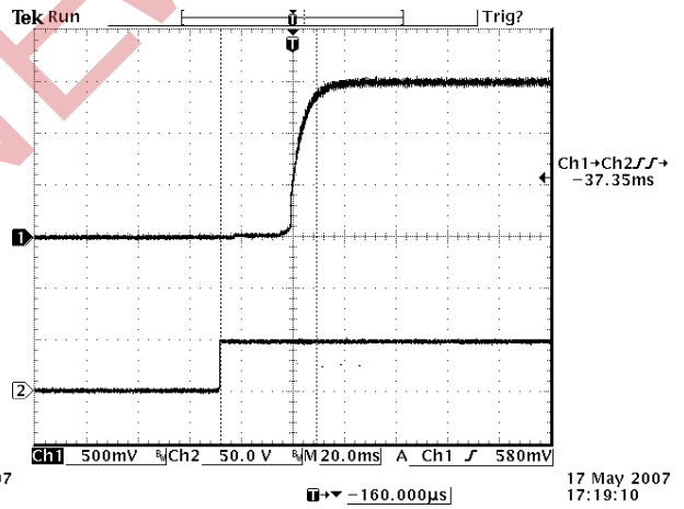
CH1: Vout CH2: Vin Vout=1.5V 100% Load at Vin=48V
