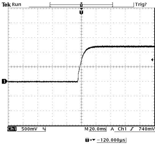
Vout=1.2V 100% Load at Vin=48V
