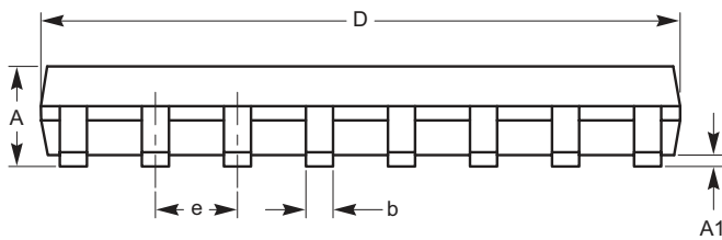
SIDE VIEW
