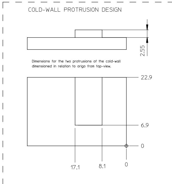
Milled protrusion areas for the baseplate in relation to the module outline.
