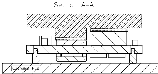
View above showing the milled protrusion for the ferrite and the two 1 mm gap pads (see hatch explanation in right box).
