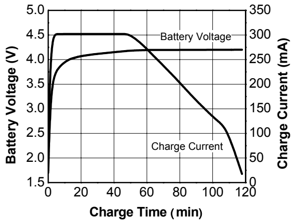
Figure 4. Complete Charge Cycle V_{IN} = 5.0V, I_{CHG} = 300mA, T_A = 25^\circ C
