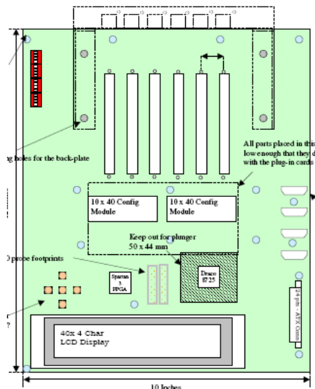
Figure 10. PEX 8713 RDK
