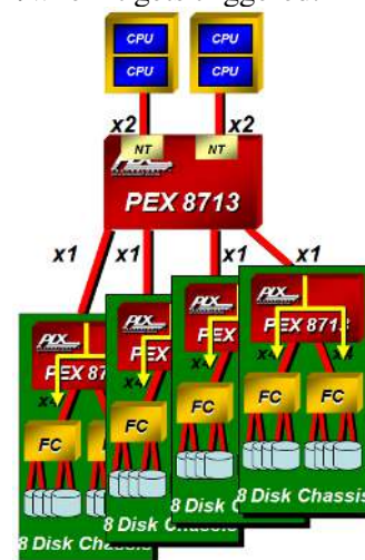
Figure 9. N+1 Failover
