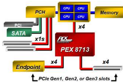
Figure 6. Host Centric Dual Upstream
