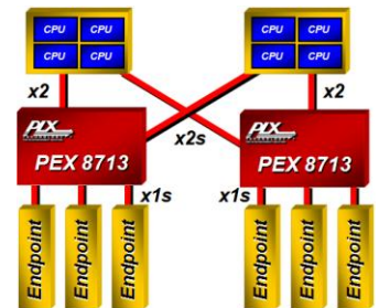
Figure 8. Host Fail-Over
