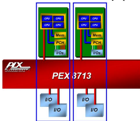
Figure 7. Multi-Host System
