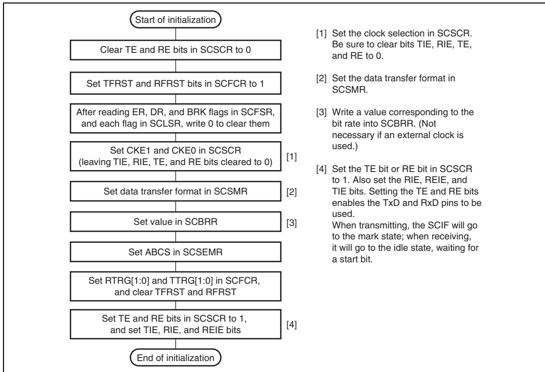
Figure 15.3 Sample Flowchart for SCIF Initialization
