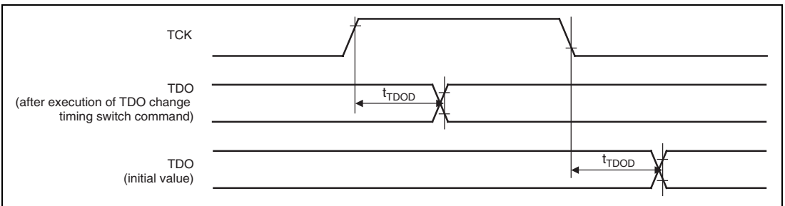
Figure 24.3 H-UDI Data Transfer Timing
