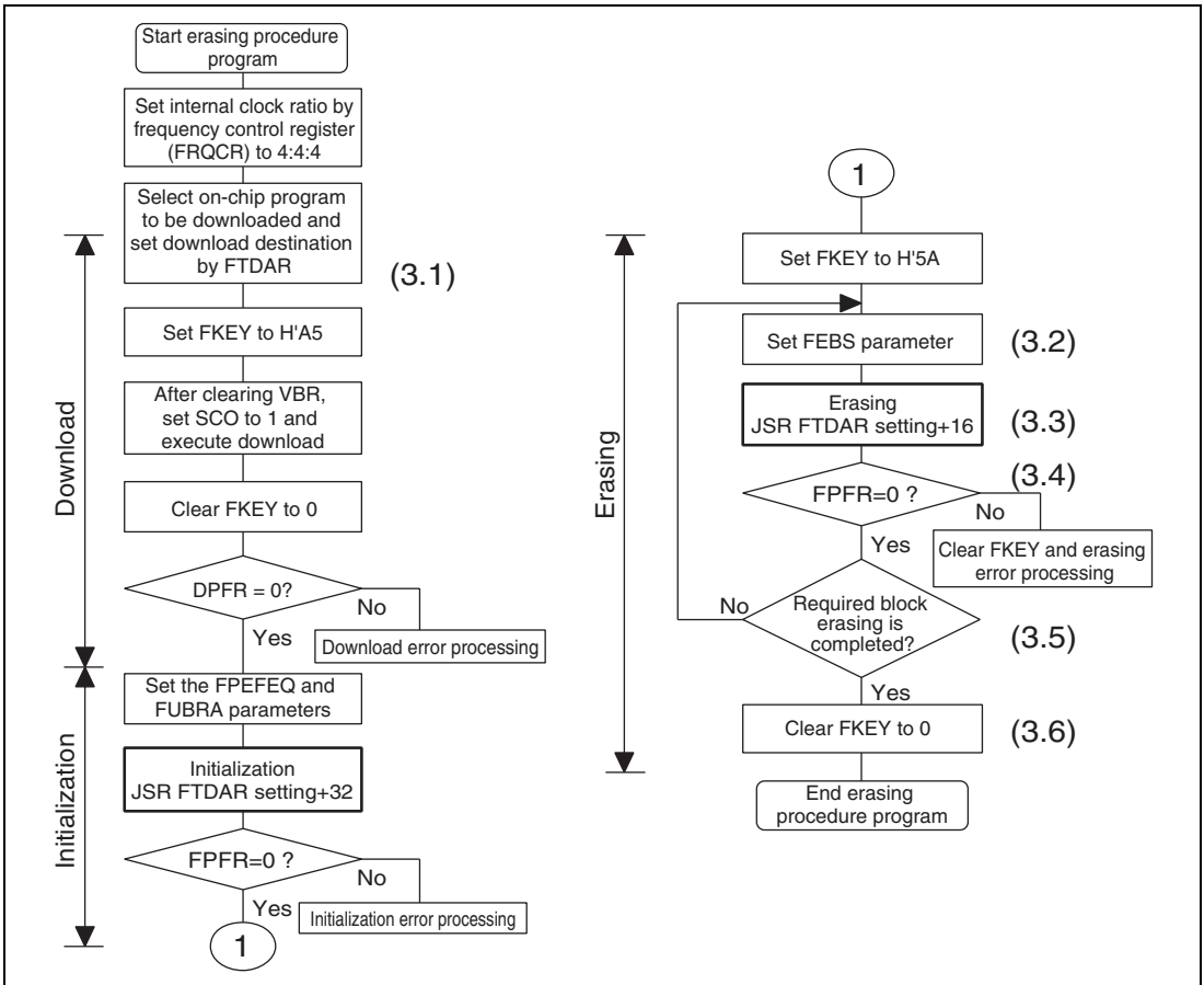
Figure 21.12 Erasing Procedure
