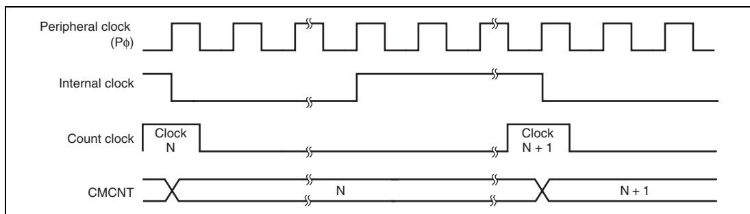
Figure 13.3 Count Timing
