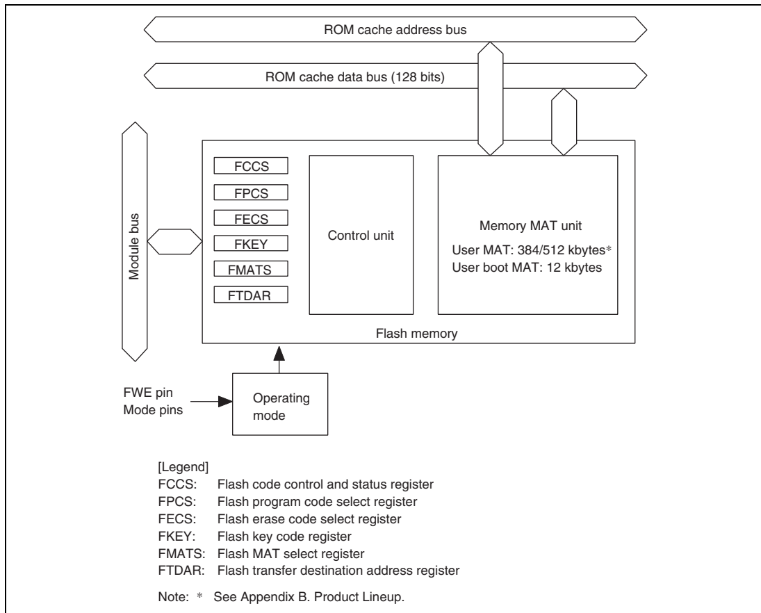
Figure 21.1 Block Diagram of Flash Memory
