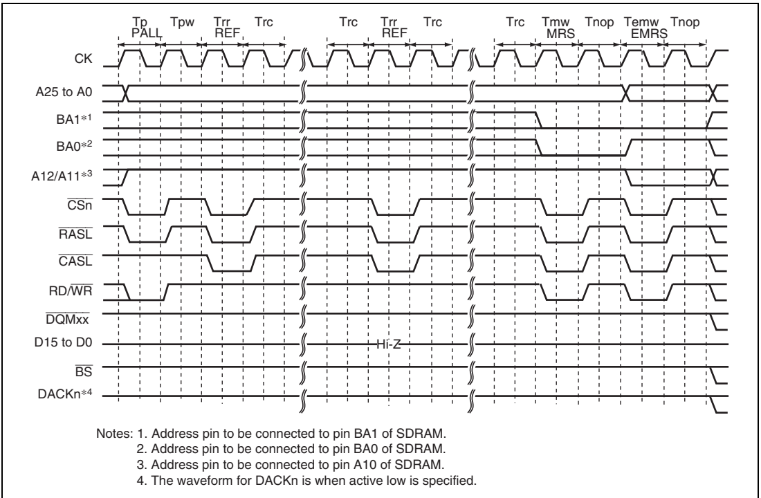
Figure 8.30 EMRS Command Issue Timing
