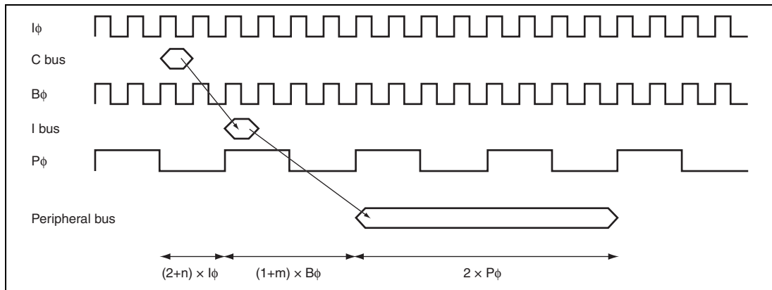
Figure 8.41 Internal Peripheral I/O Register Timing when I\phi:B\phi:P\phi = 4:4:1
