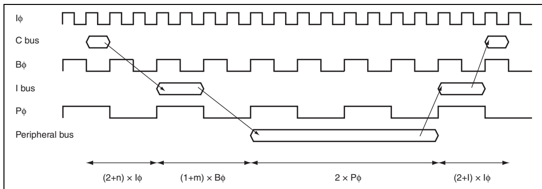
Figure 8.42 Internal Peripheral I/O Register Timing when I\phi:B\phi:P\phi = 4:2:1
