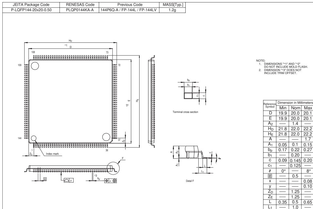
Figure C.1 FP-144LV
