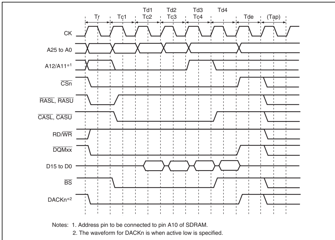
Figure 8.14 Burst Read Basic Timing (CAS Latency 1, Auto-Precharge)
