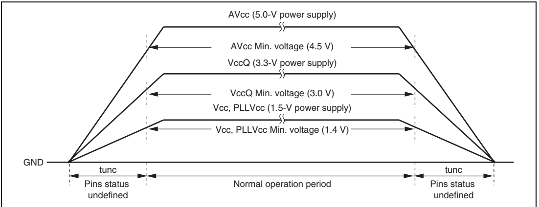
Figure 27.1 Power-on/Power-off Sequence
