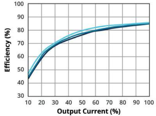
EFFICIENCY VS OUTPUT LOAD PCN2-S5-D15-S
