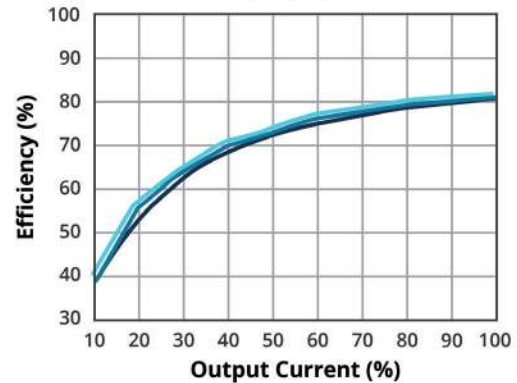
EFFICIENCY VS OUTPUT LOAD PCN2-S12-D5-S
