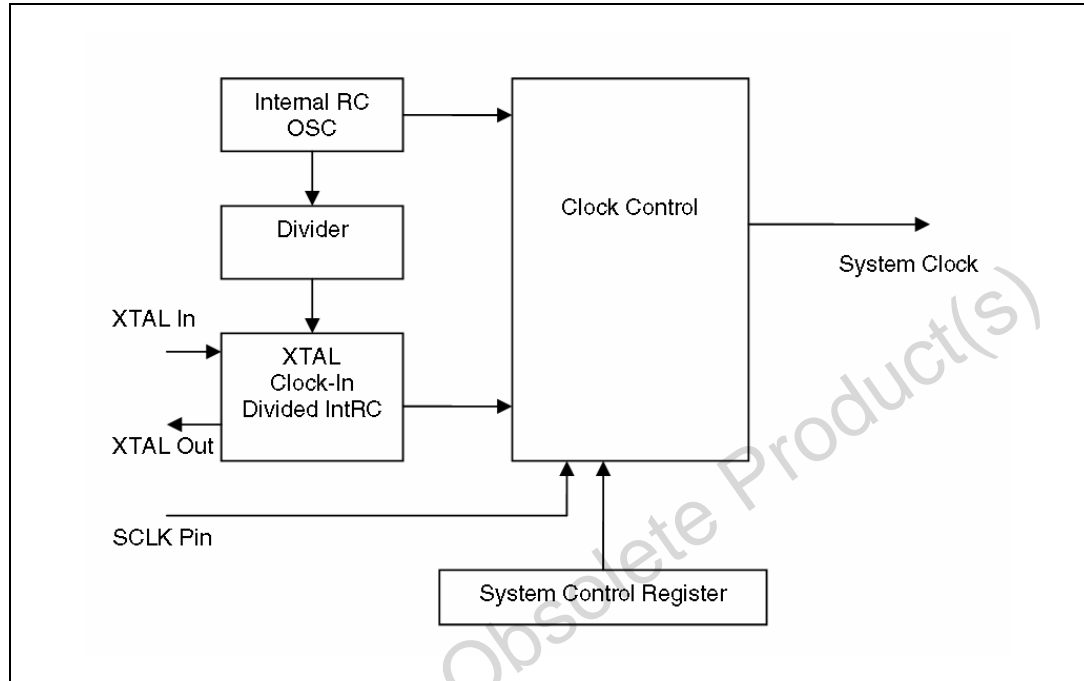
Figure 5. Clocking system
