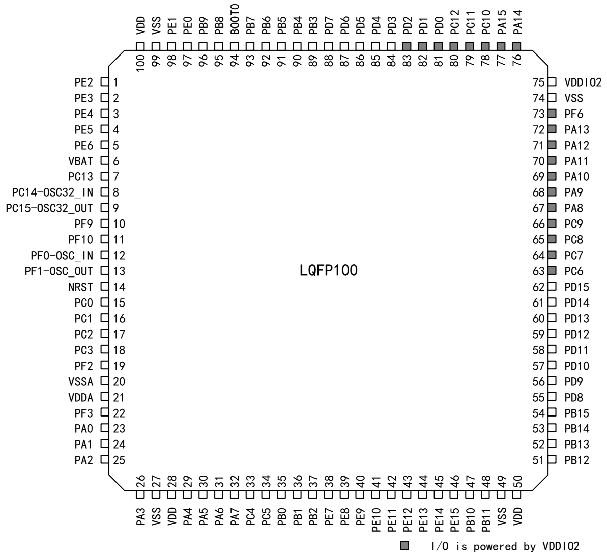
Figure. 1 Pin Distribution Diagram of APM32F072x8xB Series LQFP100
