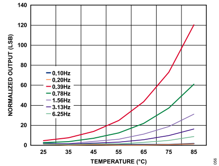
Figure 54. Typical X-Axis Output vs. Temperature at Lower Data Rates, Normalized to 100 Hz Output Data Rate, V_S = 2.5\text{ V}
