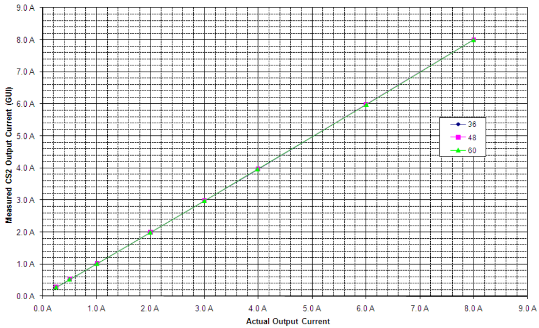
Figure 92 - Output current reading linearity
