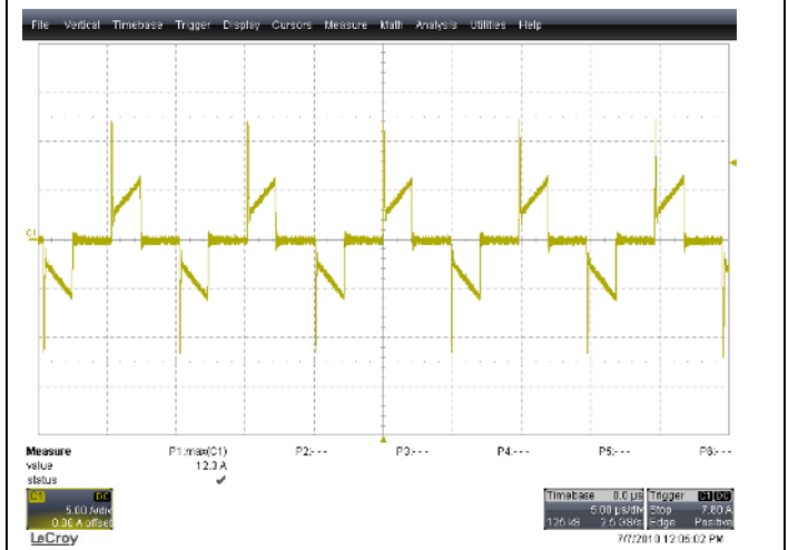
Figure 73 - Primary current at 48VDC, 8A load, 5A/div, 5us/div
