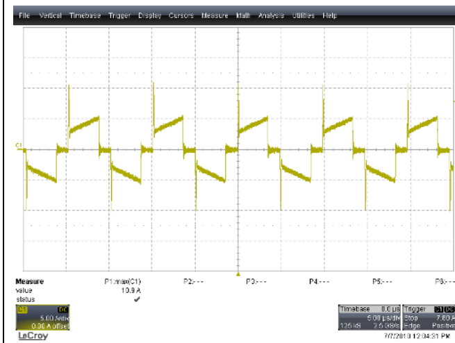
Figure 72 - Primary current at 36VDC, 8A load, 5A/div, 5us/div
