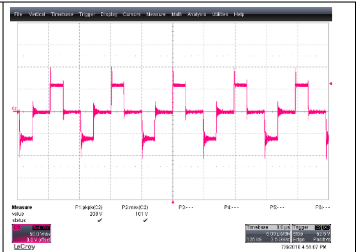
Figure 71 - Voltage across transformer primary, 60VDC, 8A load, 50V/div, 5us/div
