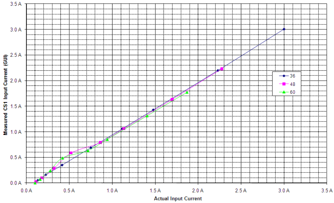
Figure 91 - Input current reading linearity
