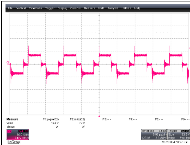
Figure 70 - Voltage across transformer primary, 36VDC, 8A load 50V/div, 5us/div
