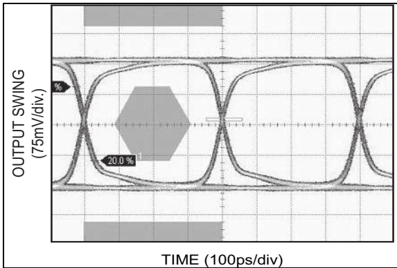
FIGURE 4-7: 2.5 Gbps Data.
