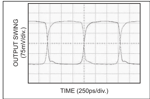
FIGURE 4-10: 625 MHz Clock.
