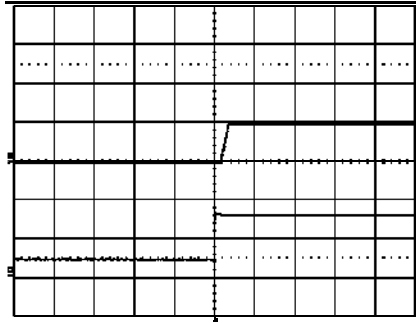
Start-up enabled by connecting V_i at: T_{ref} = +25^\circ\text{C} , I_O = 6\text{ A} resistive load, V_i = 3.3\text{ V} . Top trace: output voltage (1.0 V/div.). Bottom trace: input voltage (2 V/div.). Time scale: 20 ms/div.
