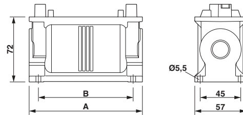
Dimensional drawing with letter dimension A
