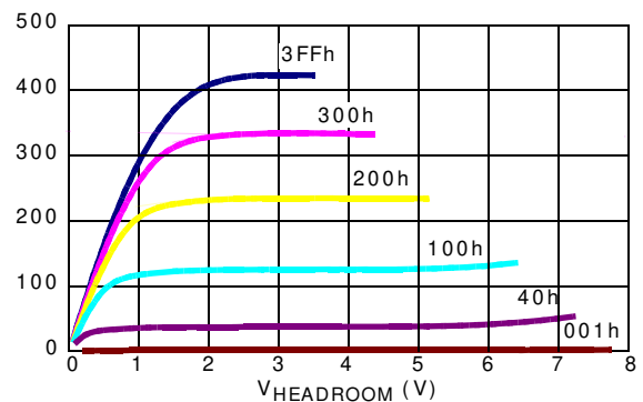
FIGURE 2. I BLUE vs P MAX vs V HEADROOM (V SO = 5.0V) (R SET = 620Ω) (1-21 = FFh), (R LOAD = 10Ω)
