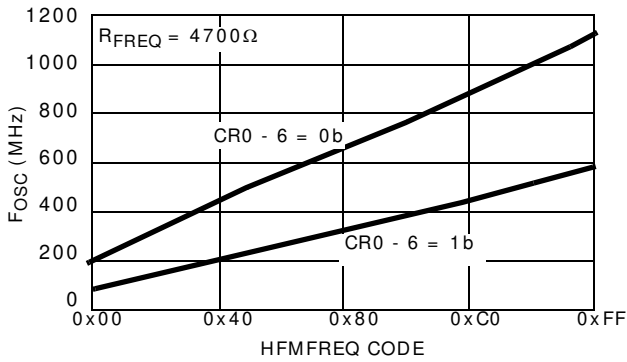
FIGURE 5. HFM CONTROL
